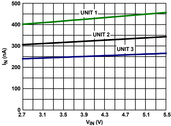
FIGURE 14. I_{IN} vs V_{IN} , THREE UNITS
