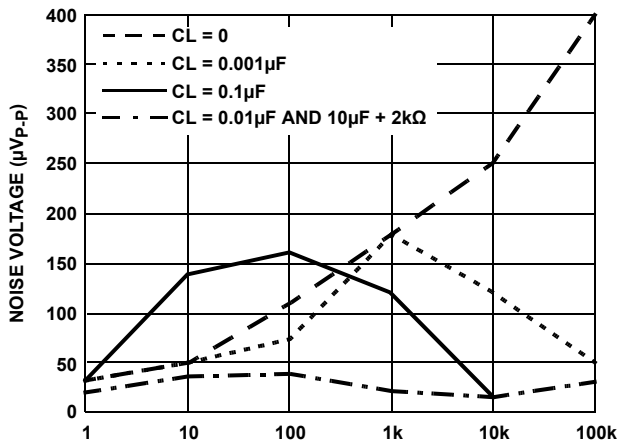
FIGURE 43. NOISE REDUCTION
