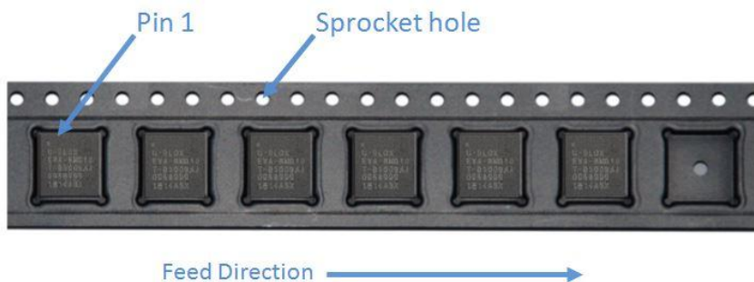
Figure 5: Orientation of EVA-8M modules on the tape
