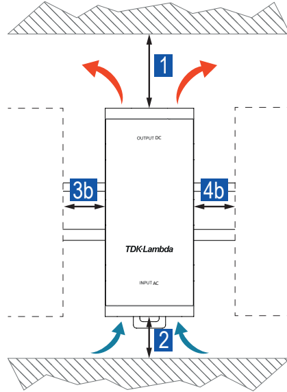
Fig. 21: Installation clearances to passive components
