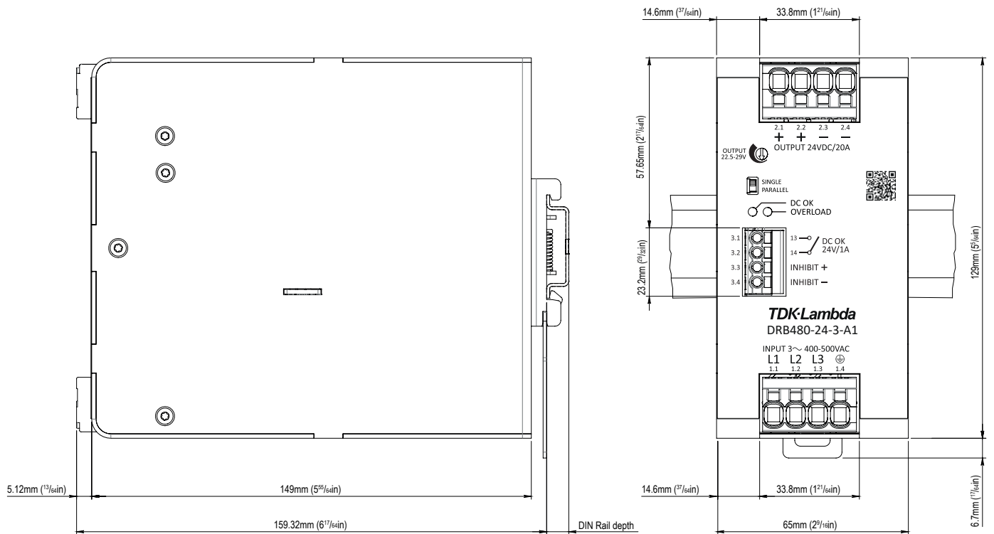
Fig. 19: Dimension drawing of DRB480-24-3-A1
