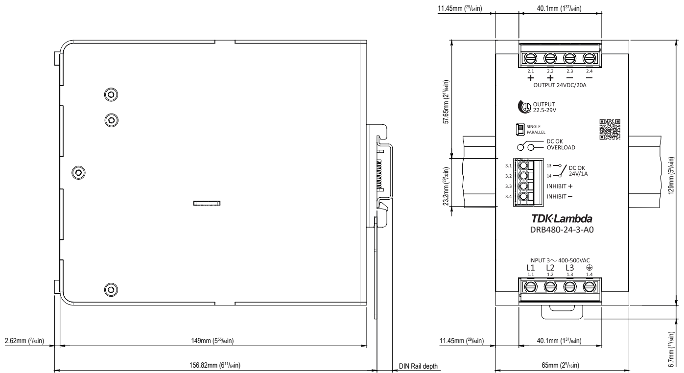
Fig. 18: Dimension drawing of DRB480-24-3-A0
