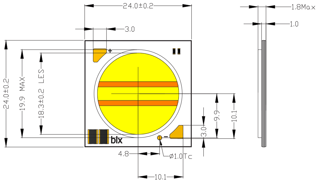
Figure 12: Mechanical Drawing
