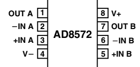
8-Lead SOIC (R Suffix)
